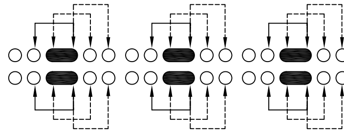
SCHEMATIC (SHORTING)
